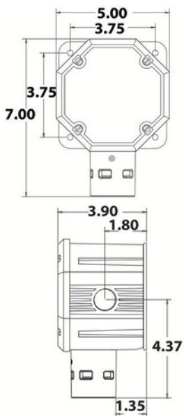
Poly Housing
