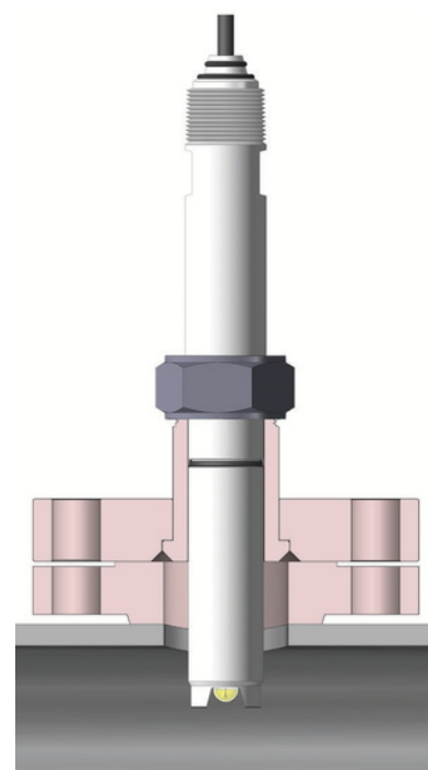
551 with Flanged Nut Lock Adapter (P/N B4951-0066)
