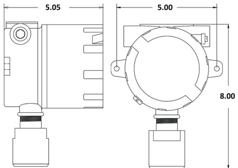
Single Sensor Aluminum/Stainless Steel Housing
